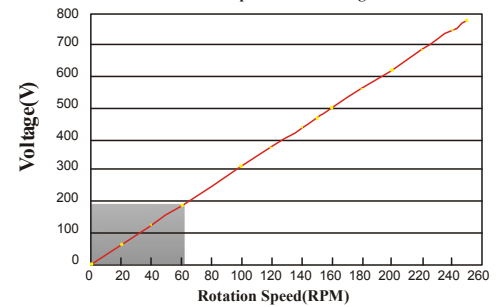
WPA-7500 PMG Open Circuit Voltage
