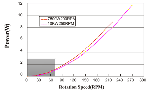
WPA-7500 PMG Power Curve
