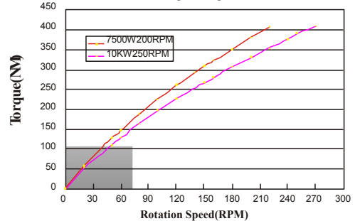
WPA-7500 PMG Input Torque Curve
